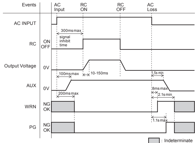
Fig.1.6 Sequence time chart by Remote ON/OFF control
