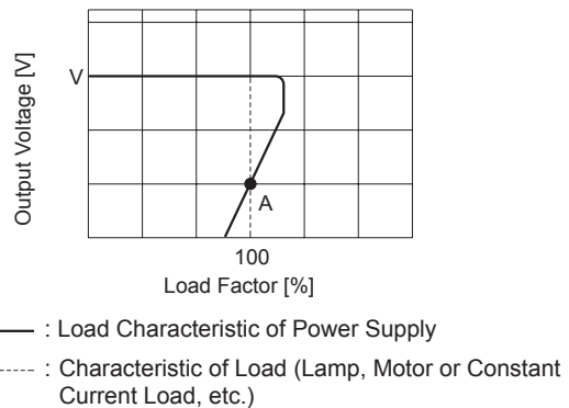
Fig.4.1 Current Foldback Characteristic
