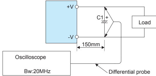
C1 : 22μF of Aluminum electrolytic capacitor
